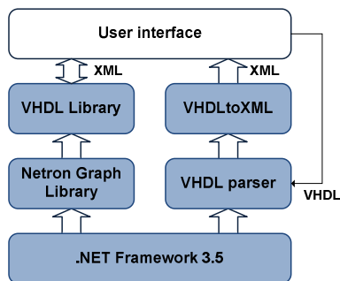
Fig. 1. The VHDLVizualizer architecture
