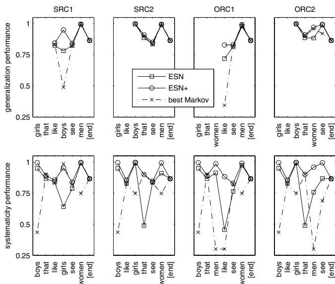
Figure 1: Performance at each point in four types of generalization (top) and systematicity (bottom) test sentences, by ESN, ESN+, and the best Markov model. Results are averaged over all test sentences of a type; those shown on the x-axis are just examples.
