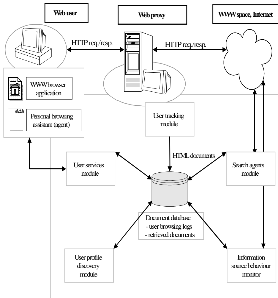
Fig. 1. Trillian architecture
