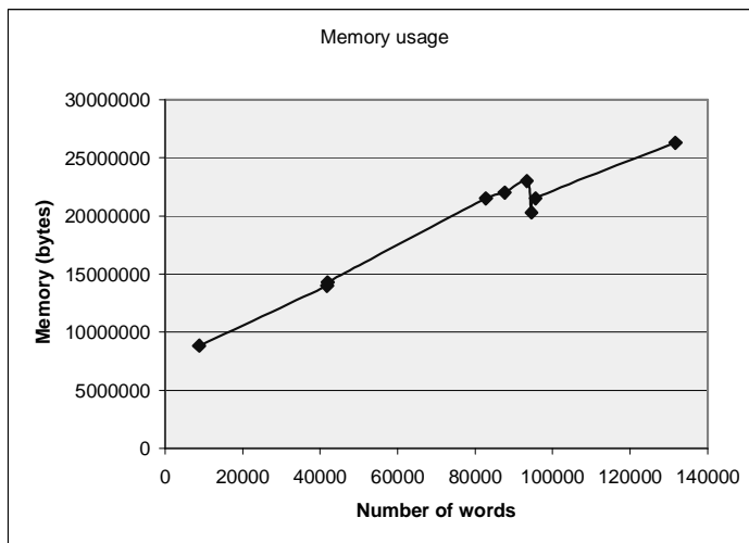
Fig. 4. Relation between number of words in document set and memory requirements
